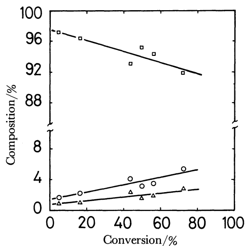
Fig. 1. Composition vs. conversion relation under 133 Pa. \square : 1-Butanethiol, \circ : butane, \triangle : 1-butene.
